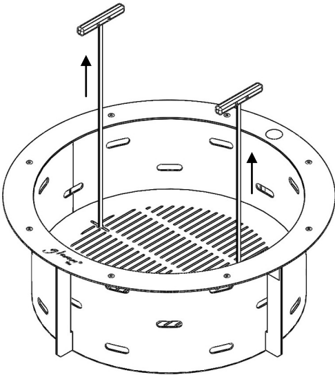
Figure 7 – Combustion zone base removal
